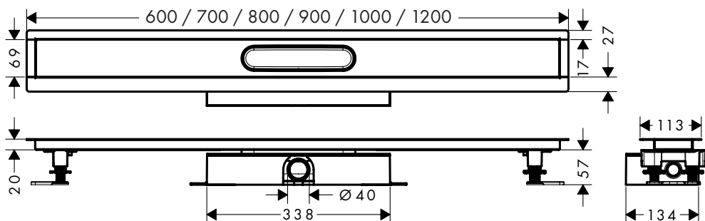
uBox universal for flat installation + installation set
