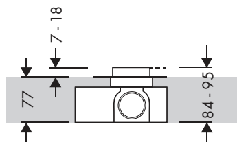
Match flat Installation
