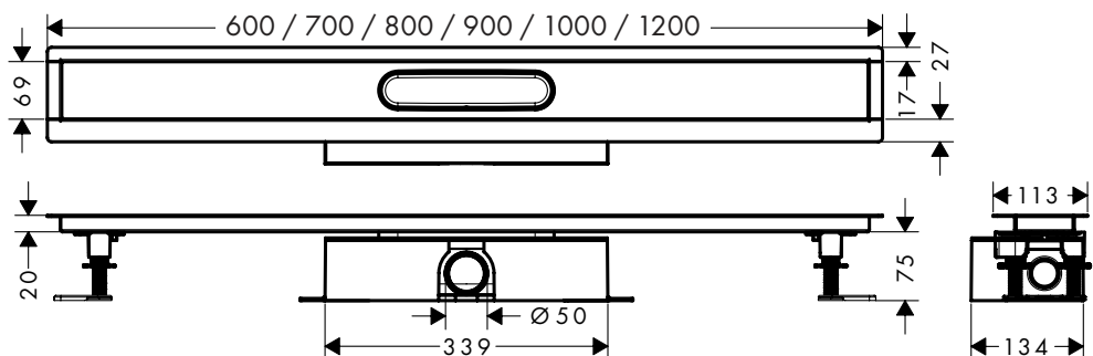
uBox universal for standard installation + installation set
