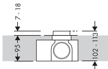
Match standard installation
