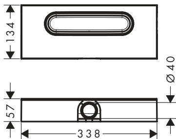
uBox flat installation
