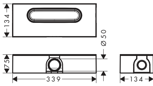
uBox standard installation
